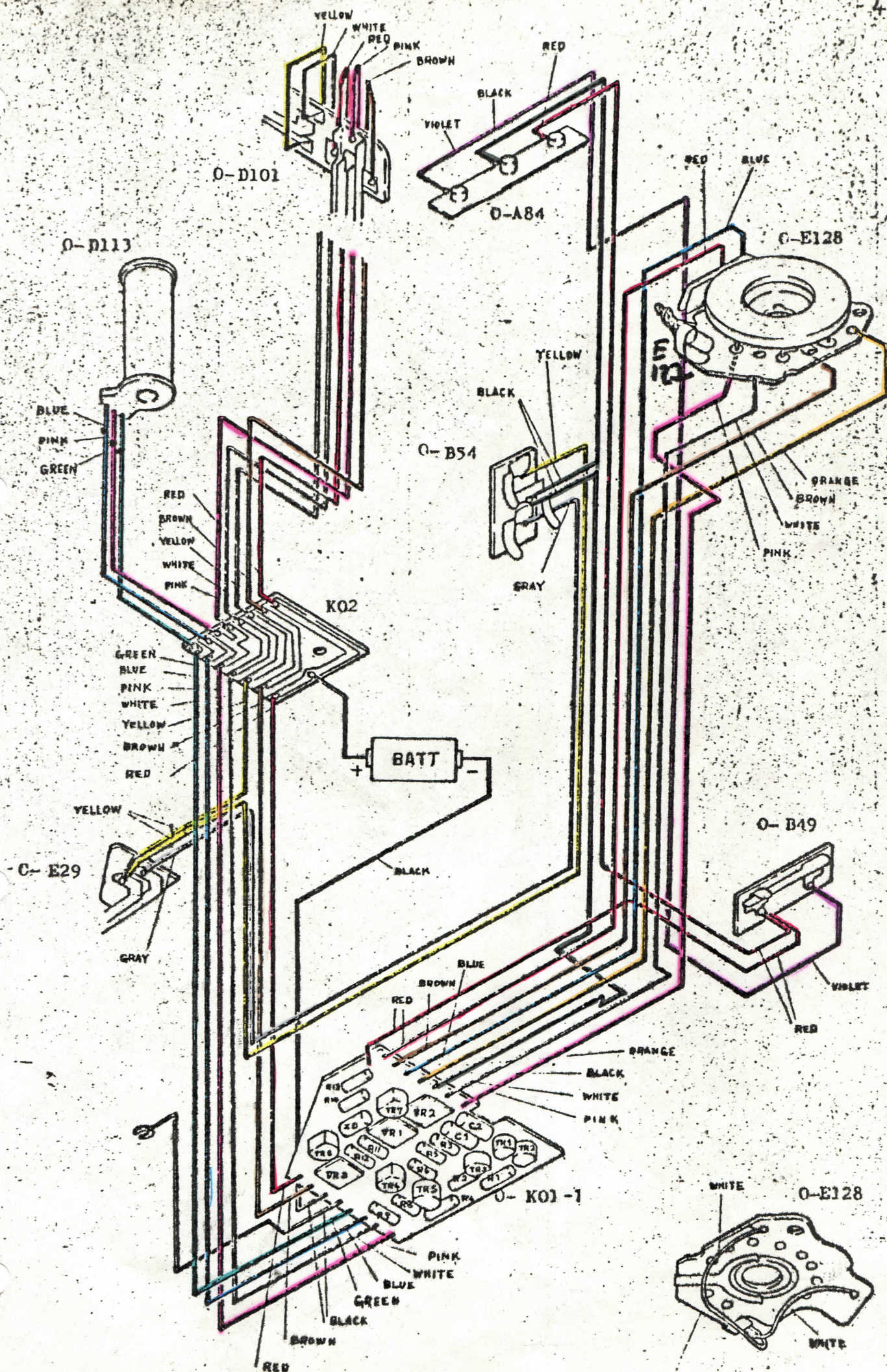
FIG. 4-111 WIRING SKETCH
