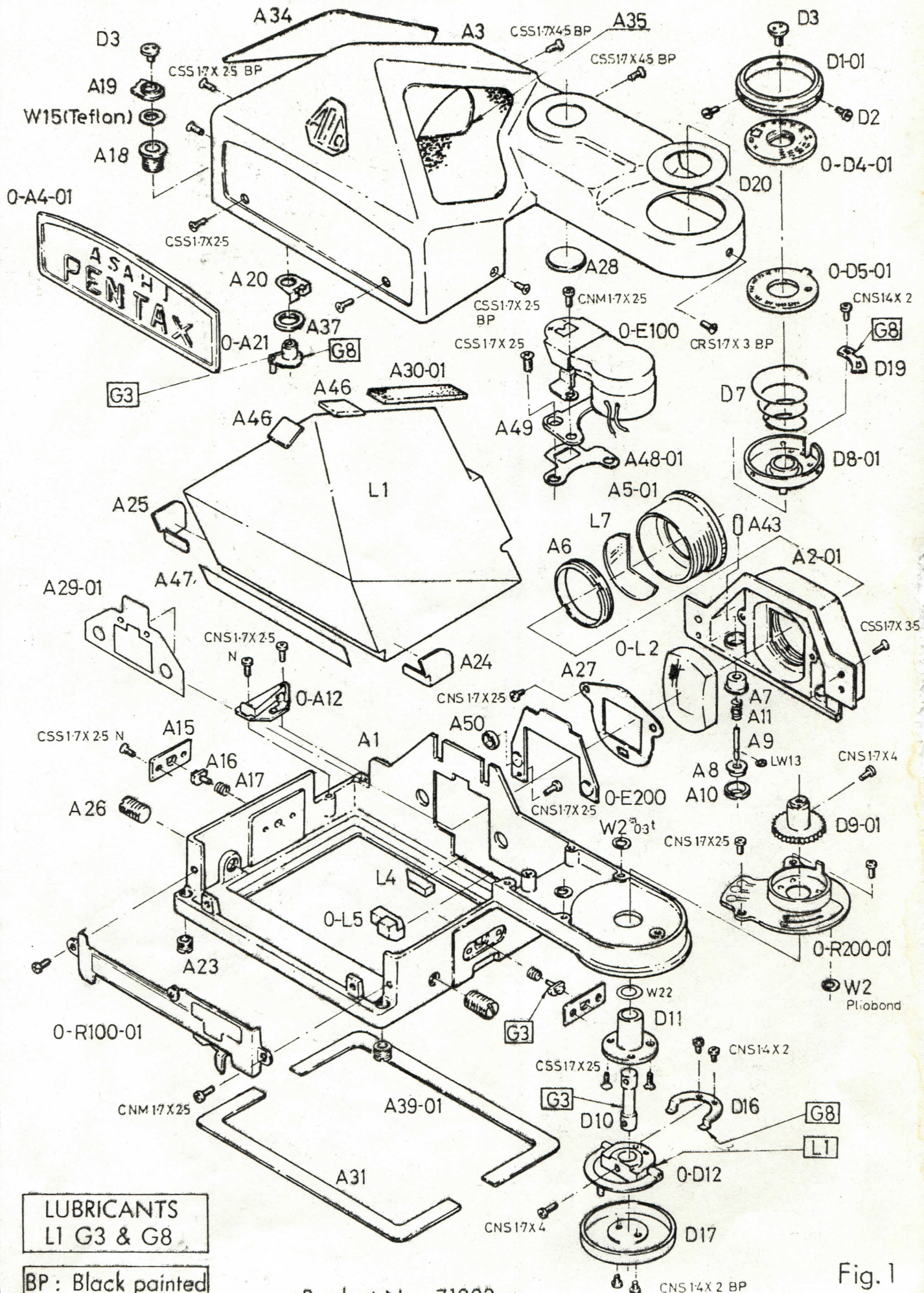
Product No. 71003 T.T.L. PENTA PRISM FINDER (MODIFIED MODEL)
